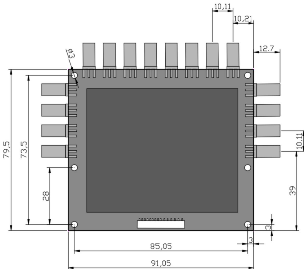
Picture No.1: Module Dimension & Hole Position
