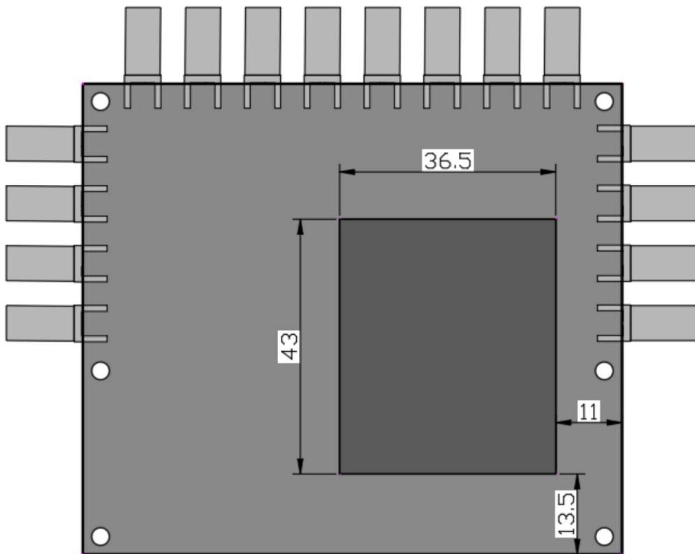
Picture No.3: Heat Sink Location
